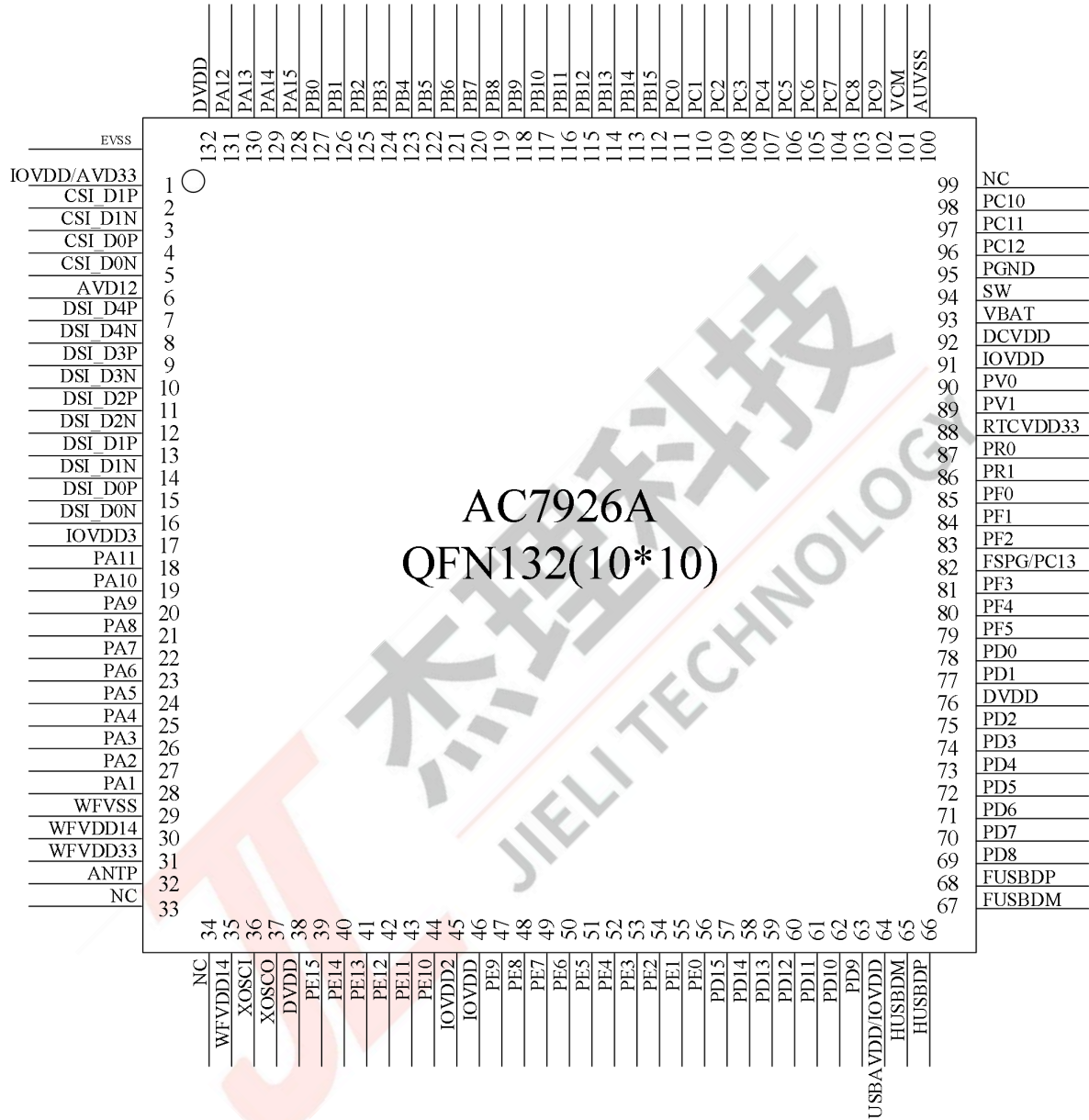
Figure 2-1 AC7926A Pin Assignment
